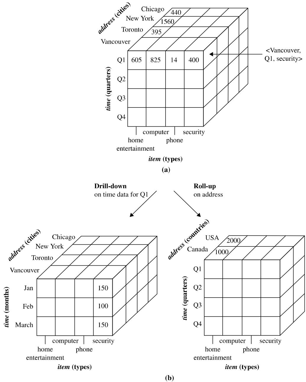
Figure 1.7 A multidimensional data cube, commonly used for data warehousing, (a) showing summarized data for AllElectronics and (b) showing summarized data resulting from drill-down and roll-up operations on the cube in (a). For improved readability, only some of the cube cell values are shown.
